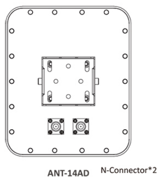
5Ghz Antenna
