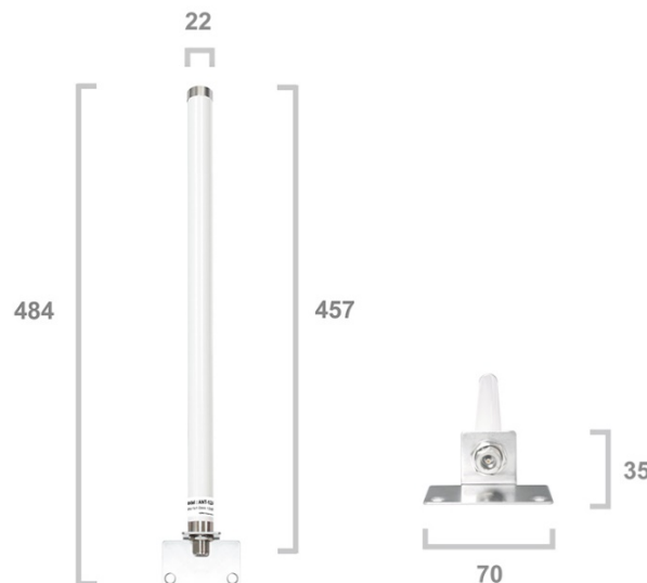
Main Unit Dimension : 457 * 22mm ( L x W ) Including bracket : 484 * 70 * 35mm ( L x W x H ) Weight : 156g / 216.5g ( Including bracket )
