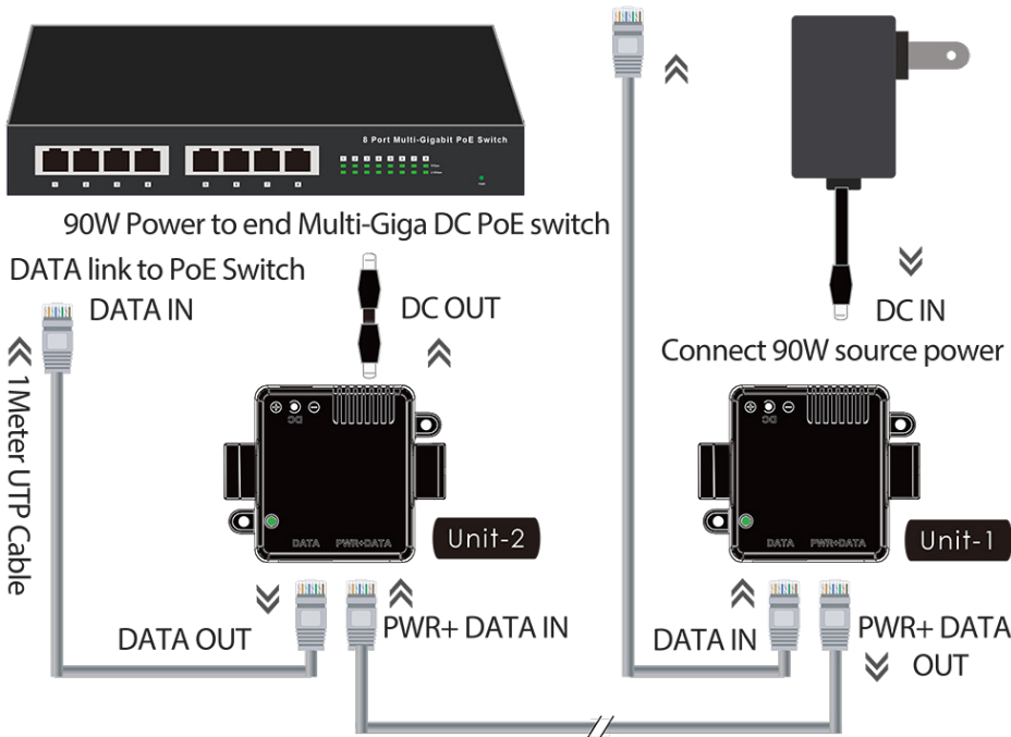
Connect data uplink from source Multi-Giga switch
