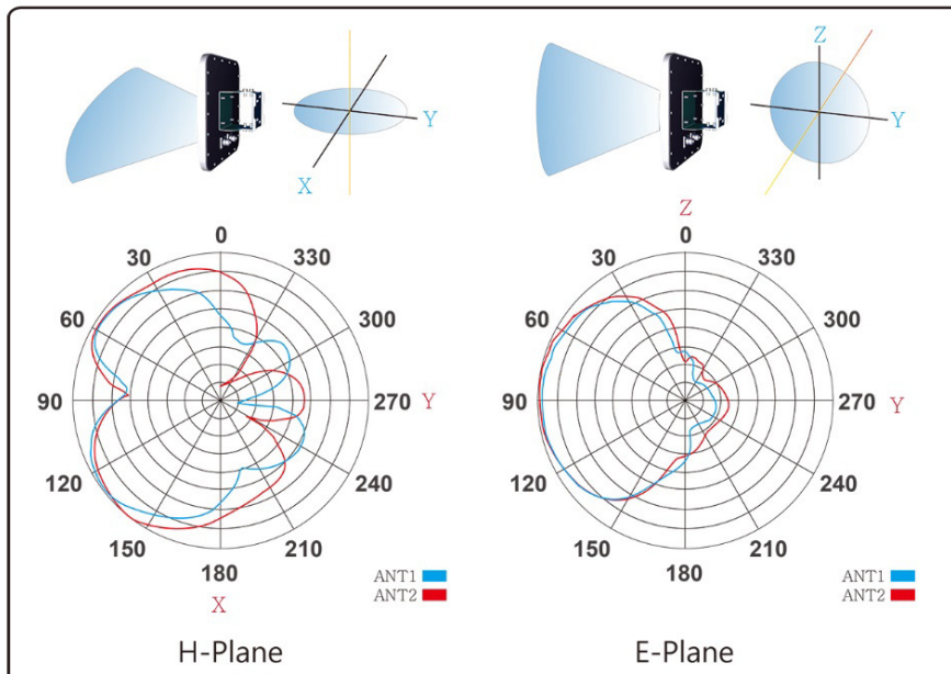
RADIATION PATTERN - 2.4Ghz 10dBi : ANT-10FD
