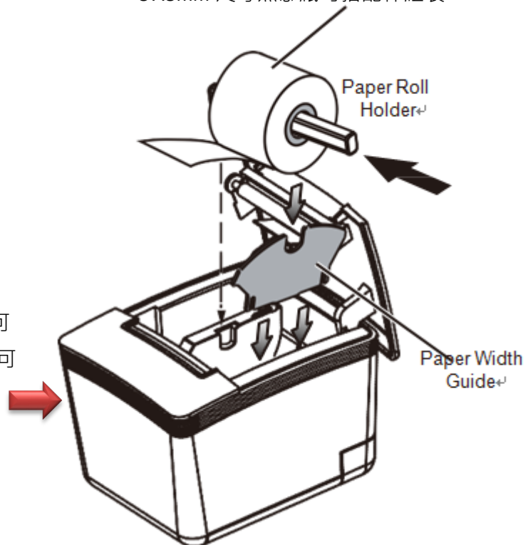
57.5mm 尺寸熱感紙可搭配附件組裝
